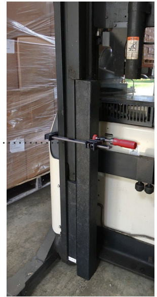
Example of mast support using both the FSS-4x4X22 and FSS-4x4x48 inner rail channel blocks.
