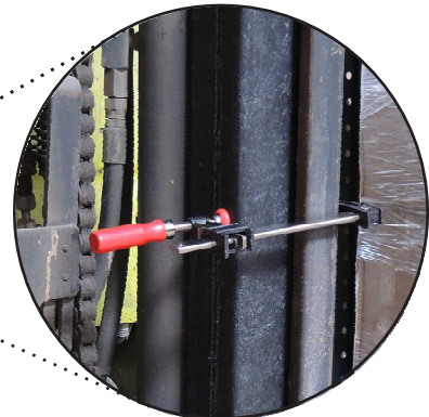
Example of a mast support using Mfg. Part# FSS-4x4x48 and Mfg. Part #FSS-Clamp.
